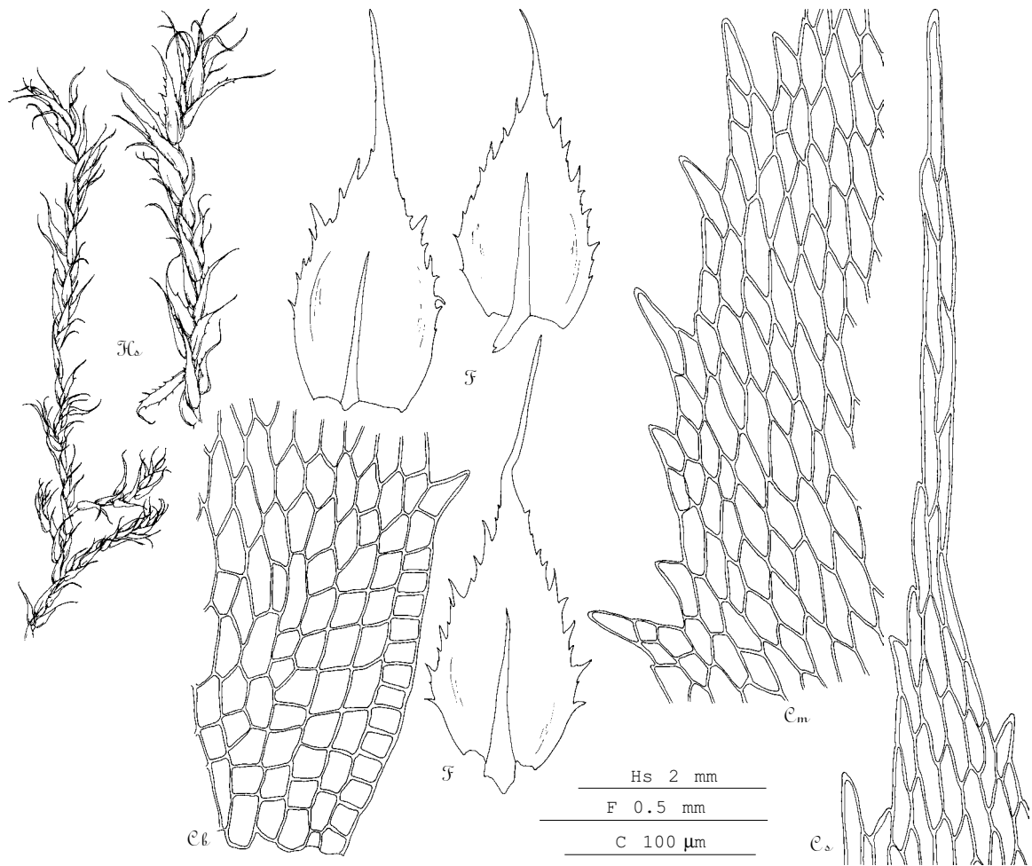
Fabronia pusilla Raddi
