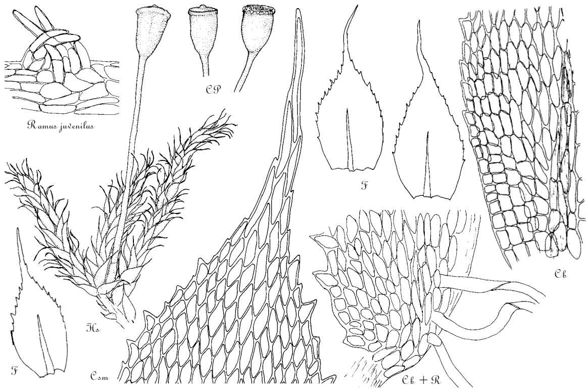
Fabronia ciliaris (Brid.) Brid.
