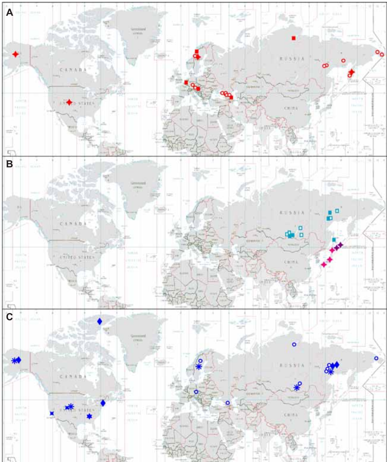
Fig. 8. Distribution of four Mieliichhoferia species known in Russia, using data on haplotypes found by Shaw (2000). A: M. mieliichhoferiana : four-pointed stars – M1 haplotype; solid squares – M2 haplotype; open circles – specimens referred to M. mieliichhoferiana by morphology. B: M. asiatica (solid squares – sequenced, E2 haplotype; open squares – referred by morphology) and M. japonica (dark stars – sequenced; light stars – referred by morphology and literature records). C: M. elongata (four-pointed star – E1 haplotype; eight-pointed star – E3 haplotype; six-pointed star – E4 haplotype; diamonds – E5 haplotype; open circles – referred by morphology). Marks outside Russia are put partly with the country/state level of exactness.
